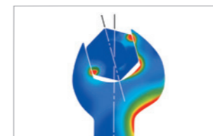
Load zones in standard-quality spanners
